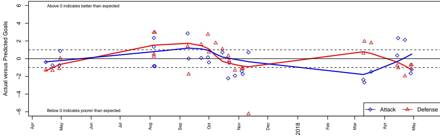
Bend FC Timbers White B04 Dots are actual minus expected GF (blue circles) and GA (red triangles). Blue line is smoothed change in attack strength. Red is smoothed change in defense strength.
